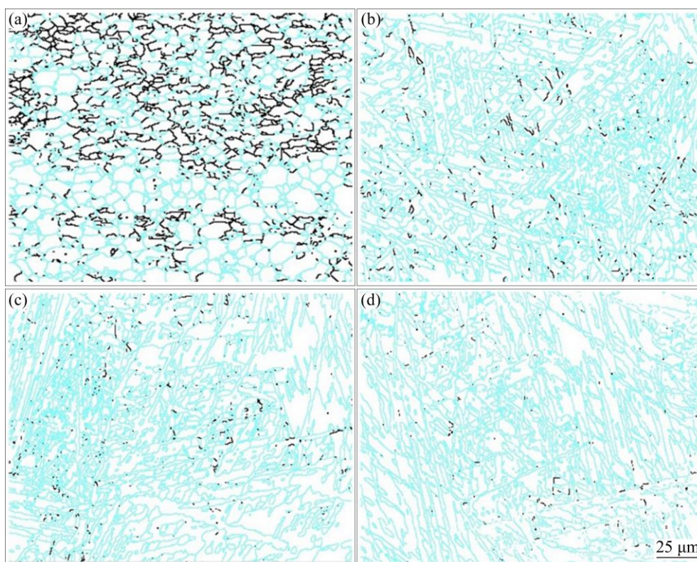
Fig. 7 GBMAD maps of \alpha phase in BM (a) and WMZ at heat inputs of 2.30 kJ/mm (b), 2.45 kJ/mm (c) and 2.62 kJ/mm (d)
