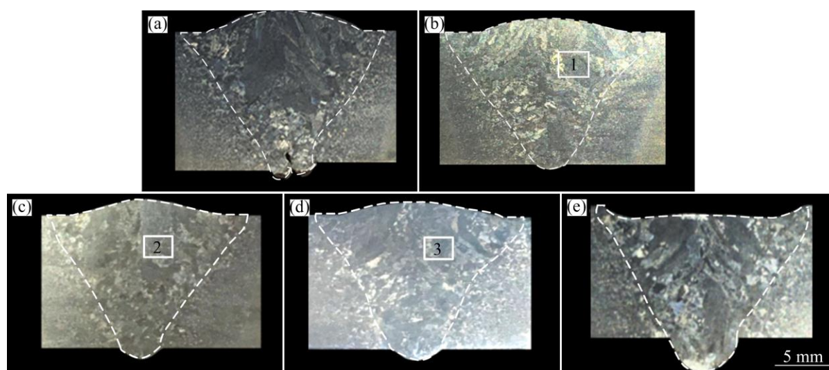
Fig. 3 Transverse cross-sections of K-TIG TC4 titanium alloy welded joint at various heat inputs: (a) 2.14 kJ/mm; (b) 2.30 kJ/mm; (c) 2.45 kJ/mm; (d) 2.62 kJ/mm; (e) 2.78 kJ/mm
