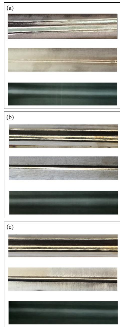
Fig. 4 Profiles of K-TIG welds at various heat inputs: (a) 2.30 kJ/mm; (b) 2.45 kJ/mm; (c) 2.62 kJ/mm
