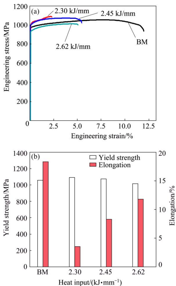
Fig. 9 Engineering stress–engineering strain curves (a), yield strength and elongation (b) of BM and WMZ at various heat inputs
