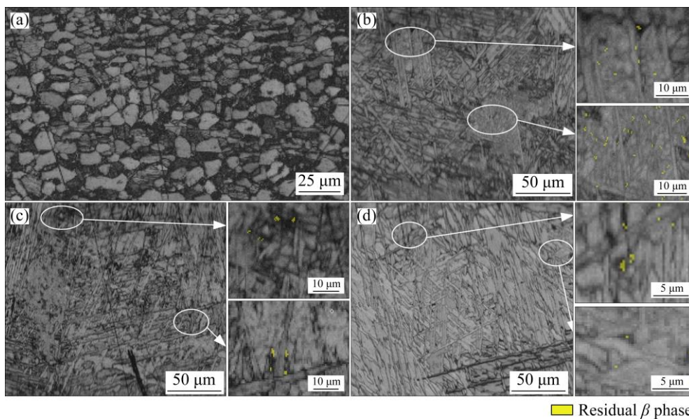
Fig. 6 Band contrast images of BM (a) and WMZ at heat inputs of 2.30 kJ/mm (b), 2.45 kJ/mm (c) and 2.62 kJ/mm (d)
