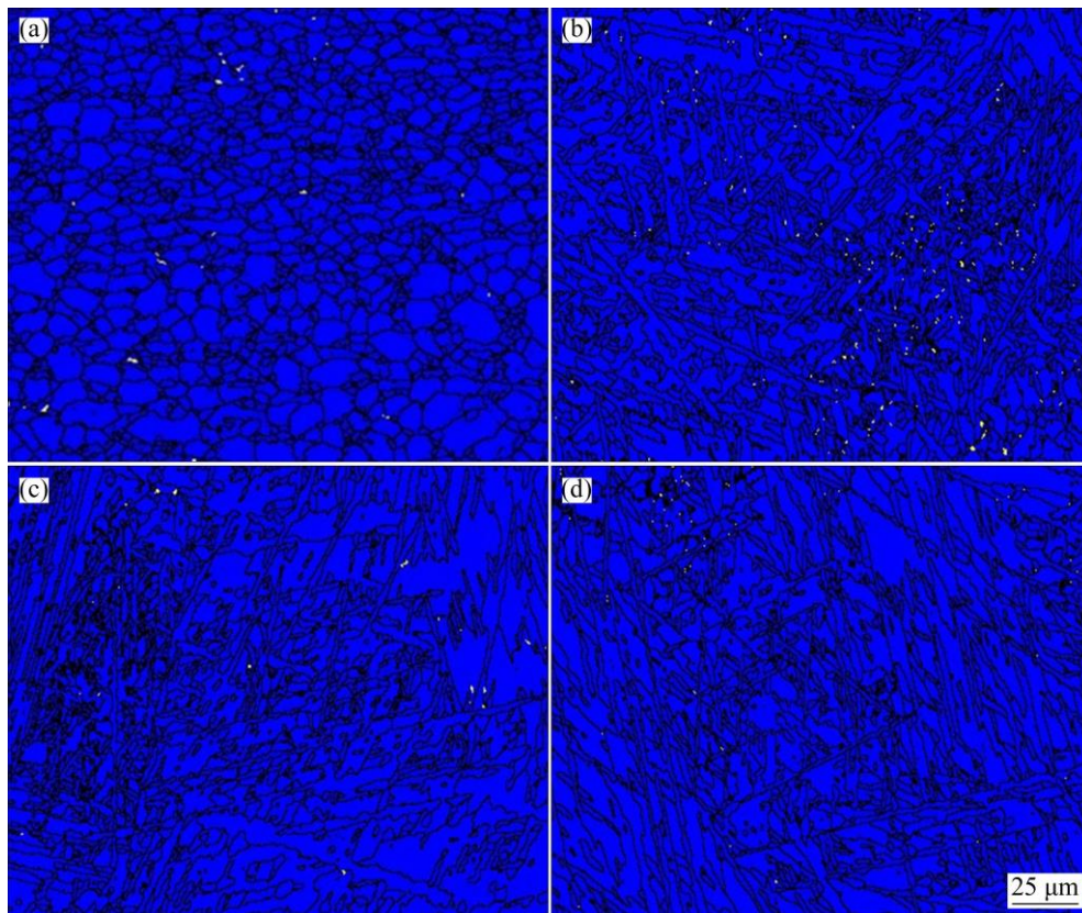
Fig. 5 Microstructures of BM (a) and WMZ at heat inputs of 2.30 kJ/mm (b), 2.45 kJ/mm (c) and 2.62 kJ/mm (d)
