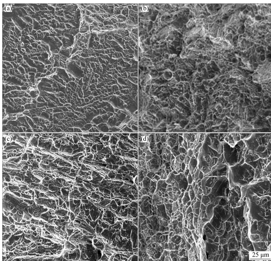
Fig. 10 SEM images of Charpy impact fracture surfaces: (a) BM; (b–d) WMZ at heat inputs of 2.30 kJ/mm (b), 2.45 kJ/mm (c) and 2.62 kJ/mm (d)
