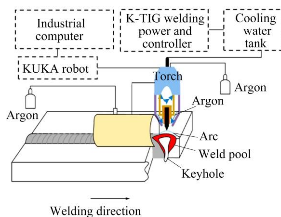
Fig. 1 Schematic diagram of K-TIG welding system
