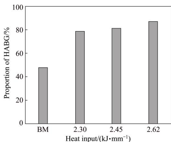
Fig. 8 High-angle GB (HAGB) proportion of \alpha phase in BM and WMZ
